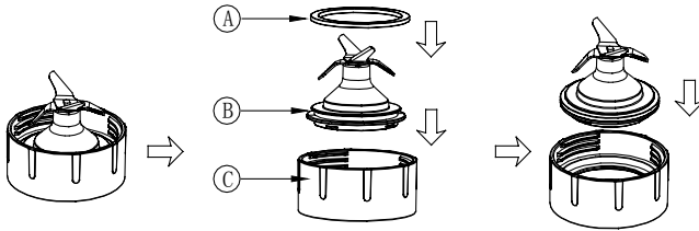
Fig 1 Assembly for Blending blade
